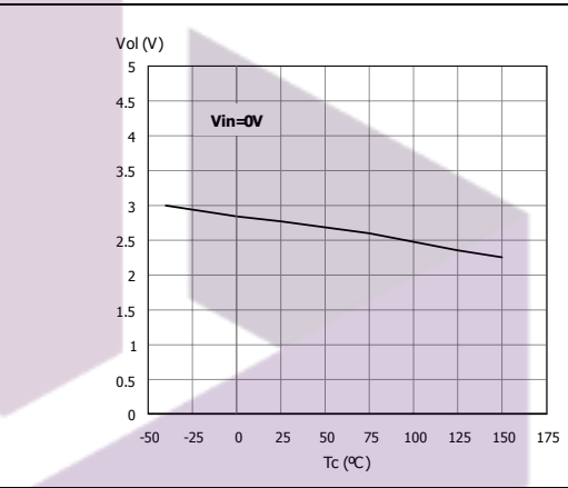
Figure 22. Openload Off state detection threshold
