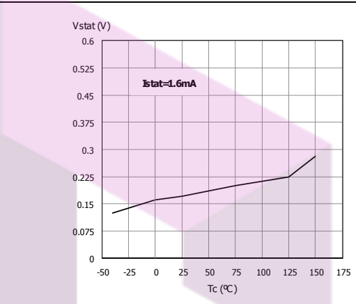
Figure 20. Status low output voltage
