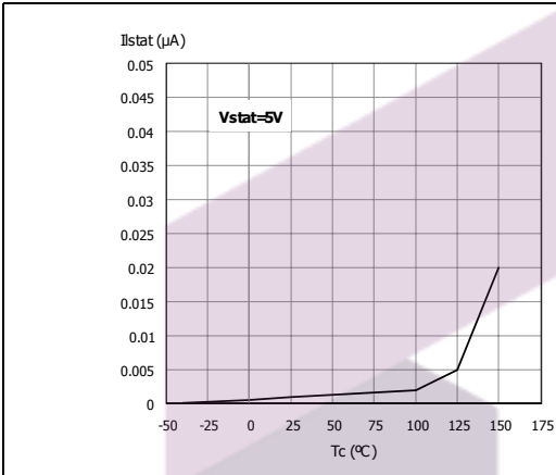
Figure 19. Status leakage current
